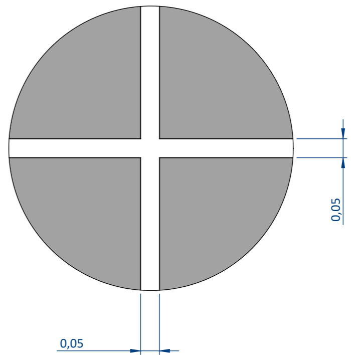
DETAIL A SCALE 100 : 1
