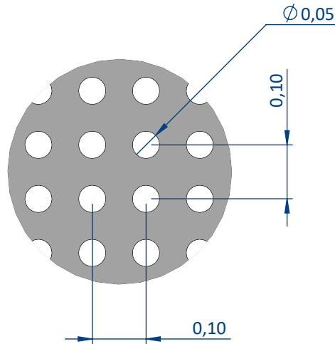
DETAIL A SCALE 100 : 1
