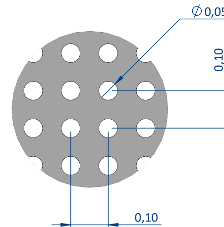
DETAIL A SCALE 100 : 1
