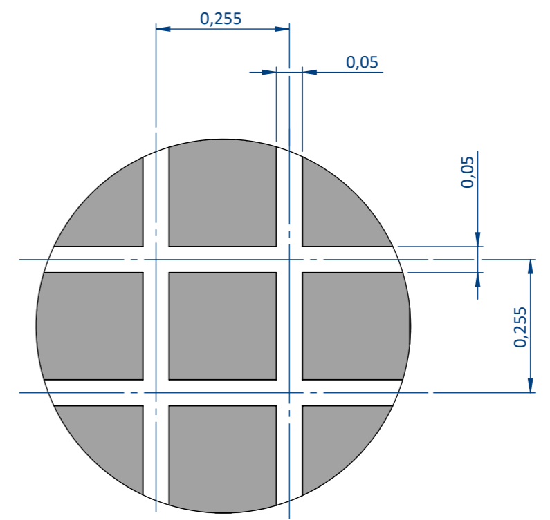
DETAIL A SCALE 100 : 1
