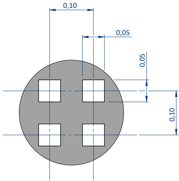
DETAIL A SCALE 200 : 1
