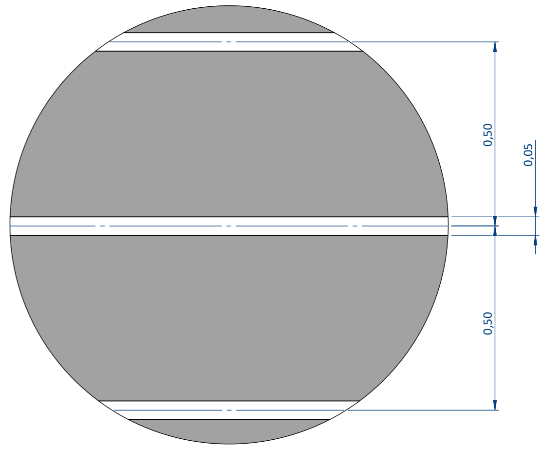
DETAIL A SCALE 100 : 1
