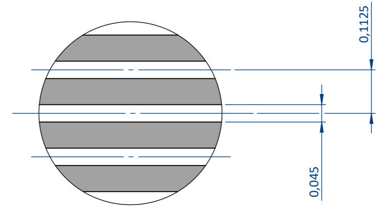
DETAIL A SCALE 100 : 1
