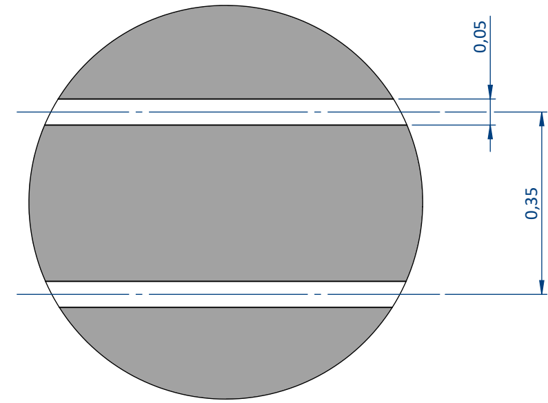
DETAIL A SCALE 100 : 1
