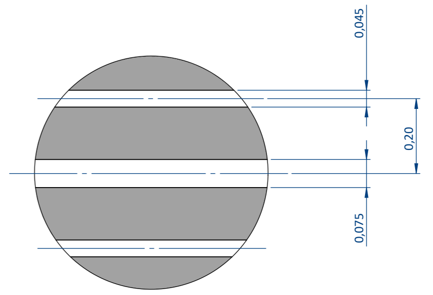
DETAIL A SCALE 100 : 1
