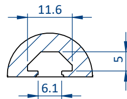
DETAIL A SACLE 1 : 1 MOUNTING: T-NUT 6MM SLOT, M4
