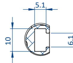
DETAIL B SCALE 1 : 1 MOUNTING : NUT M6
