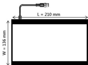
Example 1: EFFI-BL-100 T -200-1M12
