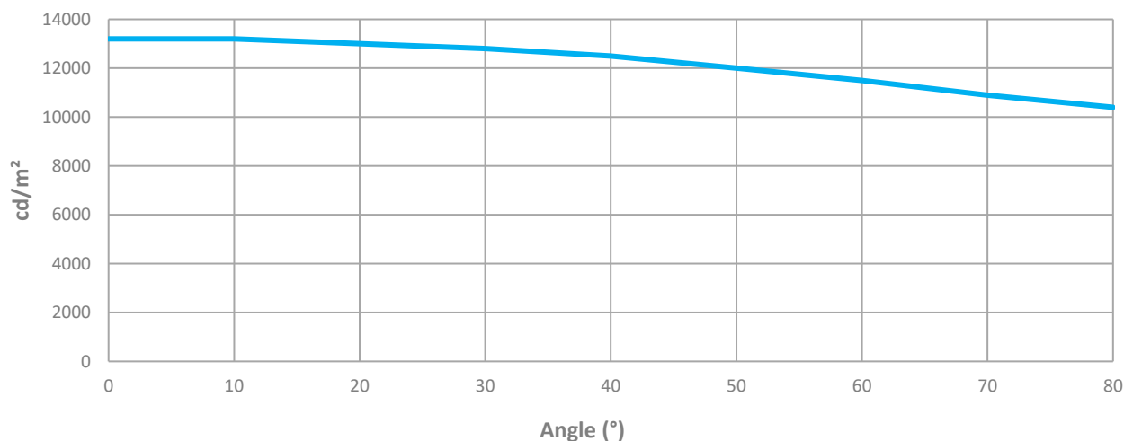
Variation of the luminance vs angle (white)
