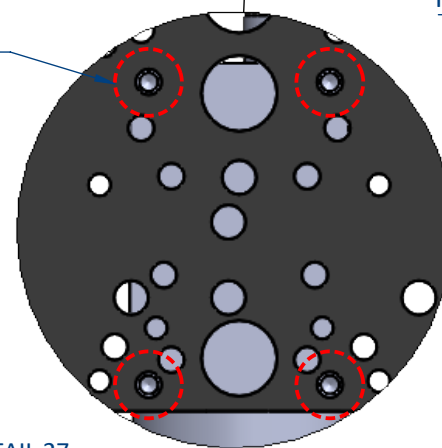
DETAIL 27 SCALE 1 : 1
