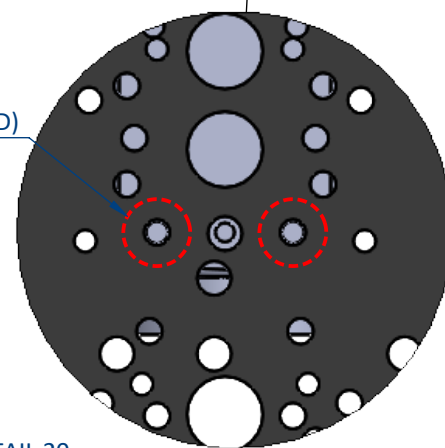
DETAIL 20 SCALE 1 : 1
