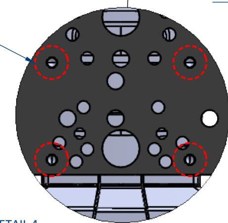
DETAIL 4 SCALE 1 : 1
